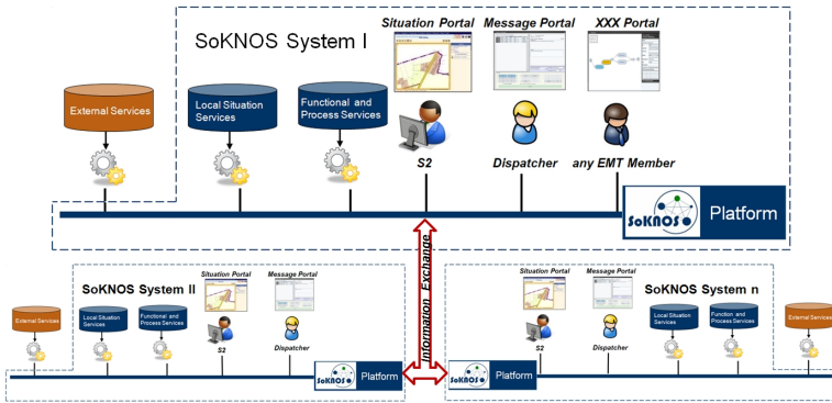
Figure 2: Each SoKNOS EMS is a distributed system; the components are connected via the SoKNOS platform. SoKNOS EMSs can be connected via the same platform functionality that is used to connect components of a single SoKNOS system.
