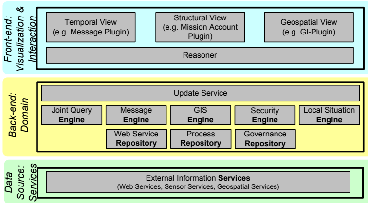
Figure 1: High-level view of the SoKNOS architecture, consisting of three decoupled layers: the data source layer, the back-end layer, and the front-end layer.
