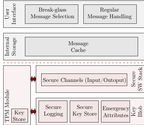
Fig. 2. Overview of the Security Infrastructure
