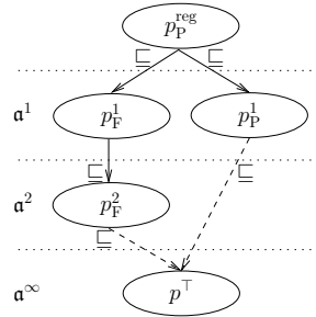
Fig. 1. A simple emergency attribute hierarchy.
