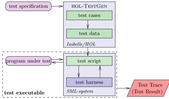
Figure 1: Overview of the Standard Workflow of HOL-TESTGEN
